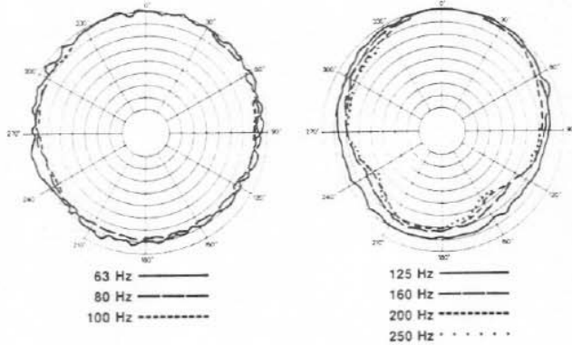
FIGURE 3 — MTL-4A Polar Response (1/3 octave, 4 volts/10 feet)
