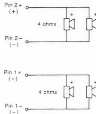
FIGURE 8 — MTL-4A Wiring Diagram
